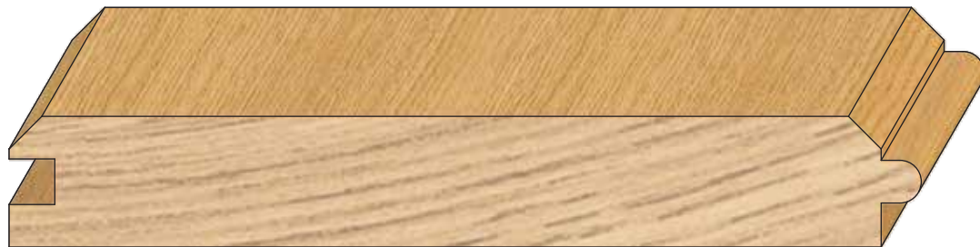
PROFILE # DIMENSION 24160TVG \frac{3}{4}'' \times 5'' (FACE)
