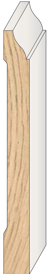
PROFILE # FJPWM618 DIMENSION 9/16" \times 5\ 1/4" \times 16'
