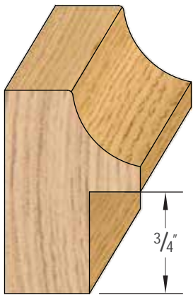
PROFILE # DIMENSION 3248ITBB 1" x 1 1/2" * 3/8" x 3/4" RABBET.
