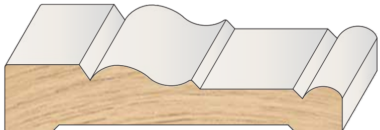
PROFILE # DIMENSION PFP22112CCA 1 1/16" x 3 1/2" x 15'
