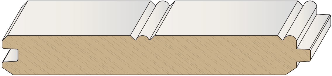
PROFILE # DIMENSION PFB18M168TVG 18mm x 5 1/4" (FACE)
