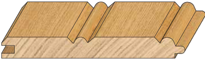
PROFILE # DIMENSION 1296TVGBD \frac{3}{8}'' \times 3'' (FACE)
