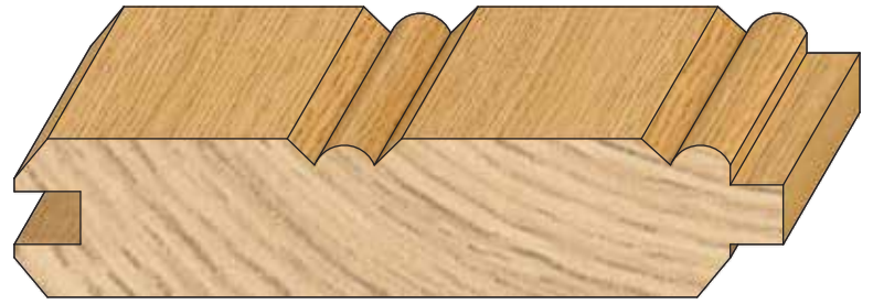
PROFILE # DIMENSION 24108TVGBD \frac{3}{4}'' \times 3\frac{3}{8}'' (FACE) * THIS PRODUCT IS REVERSIBLE.
