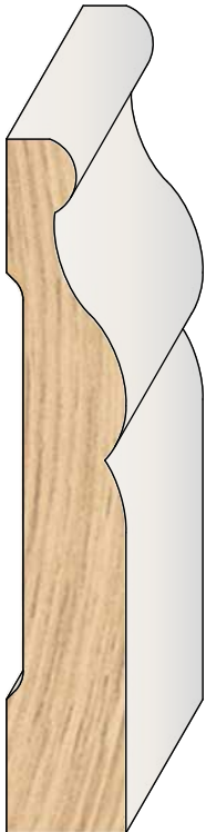
PROFILE # PFP18104CB DIMENSION 9/16" x 3 1/4" x 16'
