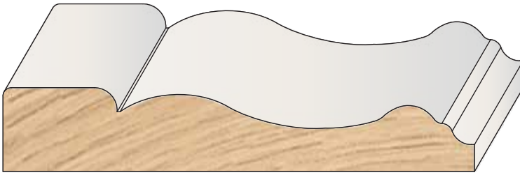
PROFILE # DIMENSION FJP20112BHCA 5/8" \times 3\ 1/2" \times 15'
