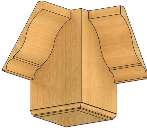
PRODUCT DESCRIPTION DIMENSION Hollow Crown Block 4" x 4" x 6 1/2"
