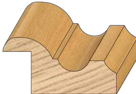
PROFILE # DIMENSION 3264PR 1" \times 2" * 1/2" \times 3/4" RABBET.
