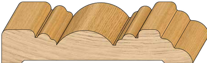
PROFILE # DIMENSION 24136BCA 3/4" X 4 1/4"
