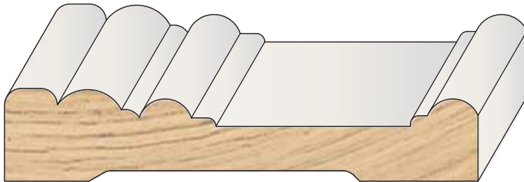
PROFILE # DIMENSION PFP22112WCA 1 1/16" x 3 1/2" x 15'
