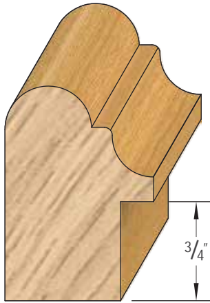
PROFILE # DIMENSION 3652BB 1 1/8" x 1 5/8" * 1/4" x 3/4" RABBET.
