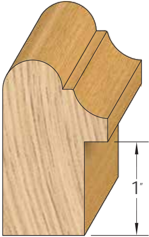
PROFILE # DIMENSION 3660BB 1 1/8" x 1 7/8" * 1/4" x 1" RABBET.
