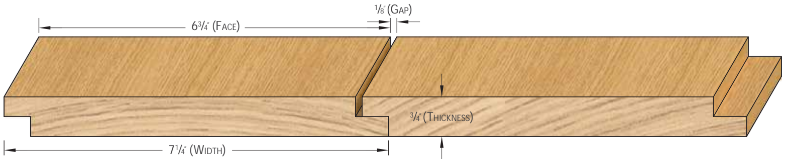
PROFILE # DIMENSION 24232SL18 3/4" x 7 1/4" * 6 3/4" FACE, 1/8" GAP
