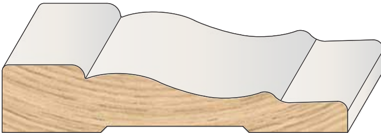
PROFILE # DIMENSION PFPWM444 1\ 1/16" \times 3\ 1/2" \times 17'
