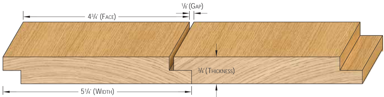
PROFILE # DIMENSION 24168SL18 3/4" x 5 1/4" * 4 3/4" FACE, 1/8" GAP
