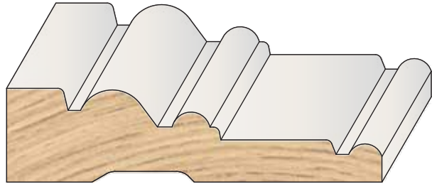
PROFILE # DIMENSION PFP2288ECA 1 1/16" x 2 3/4" x 15'
