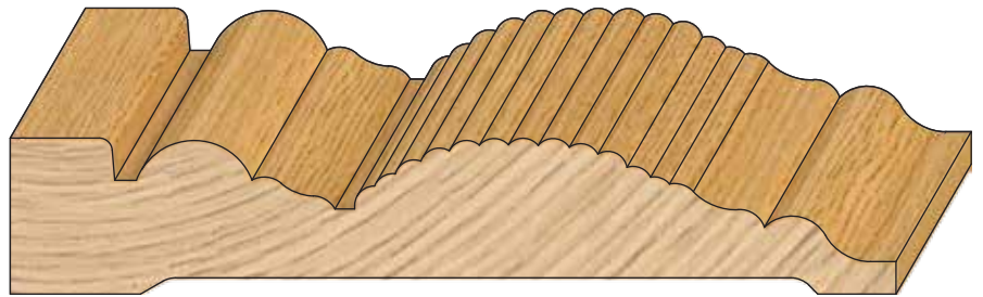
PROFILE # DIMENSION 24136RDCA 3/4" X 4 1/4"
