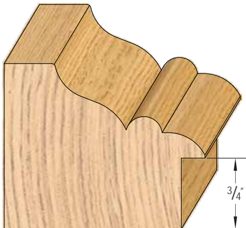
PROFILE # DIMENSION 5668BB 2 1/8" x 1 3/4" * 1/4" x 3/4" RABBET.
