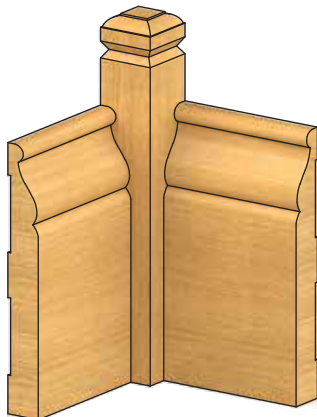
PRODUCT DESCRIPTION DIMENSION Inside - Routed Base Block 1 1/8" x 1 1/8" x 7" 1 1/8" x 1 1/8" x 10"
