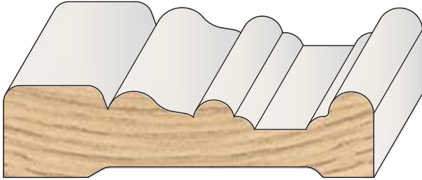
PROFILE # DIMENSION PFP2288CA 1 1/16" x 2 3/4" x 15'
