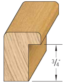
PROFILE # DIMENSION 2432EGBB 3/4" x 1" * 1/4" x 3/4" RABBET.
