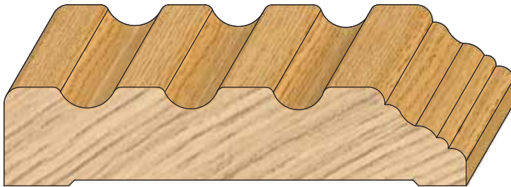
PROFILE # DIMENSION 24112FCA 3/4" X 3 1/2"
