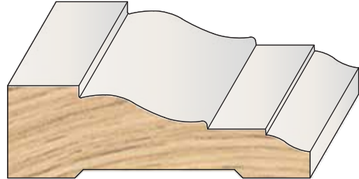
PROFILE # DIMENSION FJPWM366 1 1/16" x 2 1/4" x 14'
