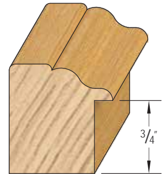
PROFILE # DIMENSION 3436BB 1 1/16" x 1 1/8" * 3/16" x 3/4" RABBET.
