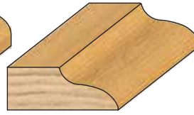
PROFILE # DIMENSION 1026S 5/16" X 1 3/16"
