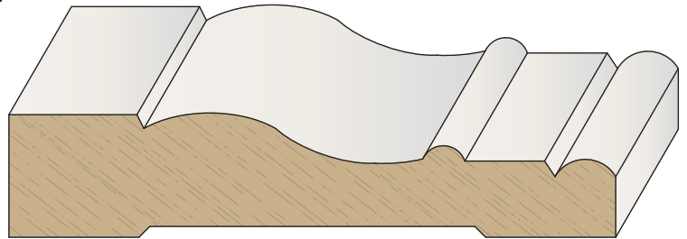
PROFILE # DIMENSION PFB18M112ULCA 18mm x 3 1/2"
