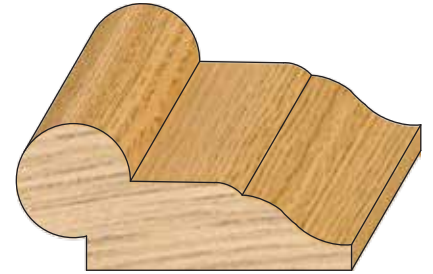
PROFILE # DIMENSION 2456PM 3/4" \times 1 3/4"
