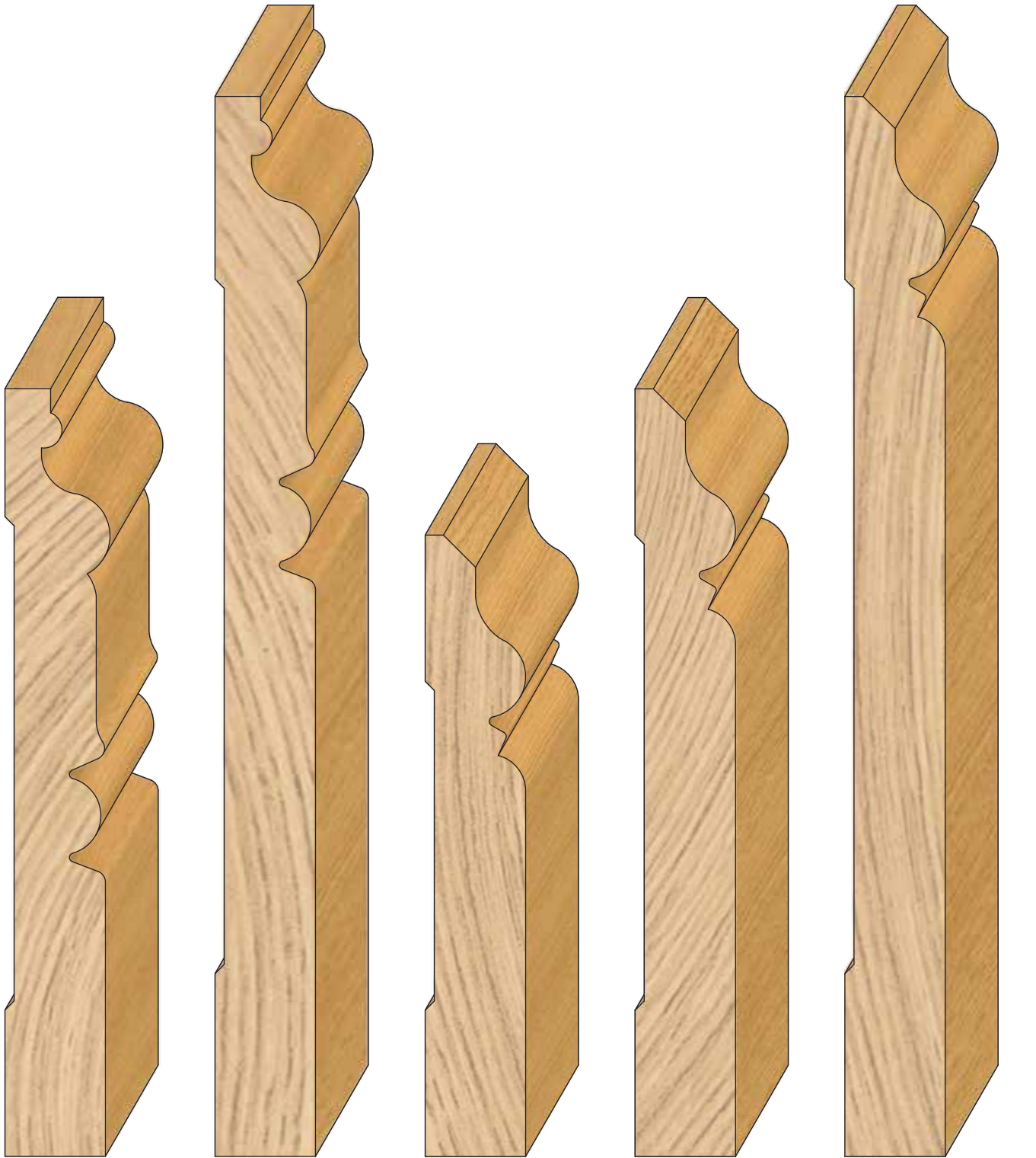
PROFILE # DIMENSION 22168EB 1 1/16" X 5 1/4"
