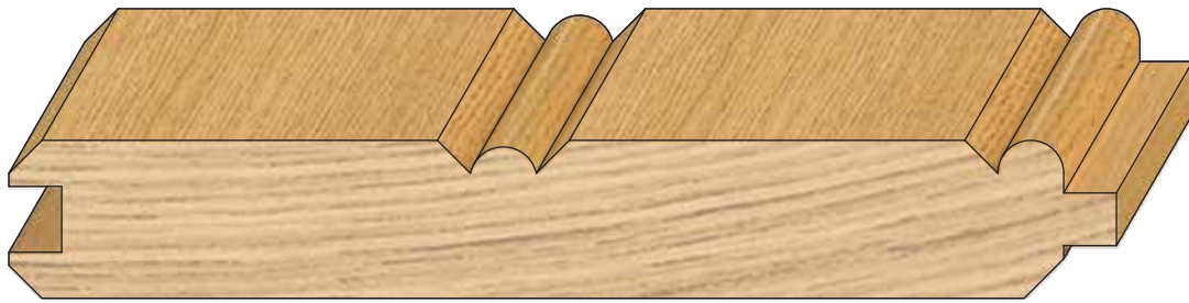
PROFILE # DIMENSION 24160TVGBD \frac{3}{4}'' \times 5'' (FACE) * THIS PRODUCT IS REVERSIBLE.
