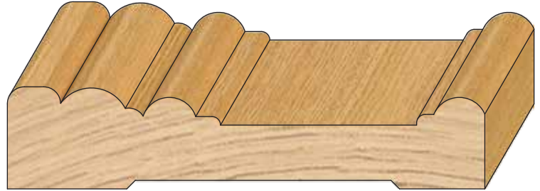
PROFILE # DIMENSION 24112WCA 3/4" x 3 1/2"
