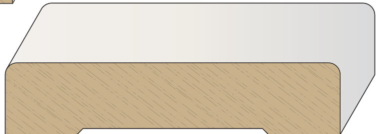
PROFILE # DIMENSION PFB24112R18CA 3/4" x 3 1/2"
